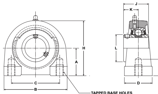
TAPPED BASE HOLES
