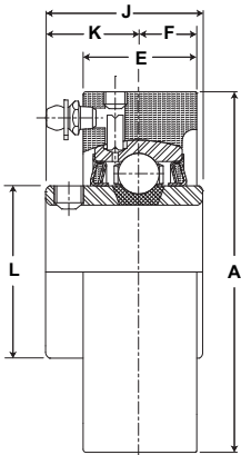
PVR x 7xx Cylindrical Cartridge Assembly
